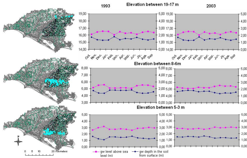
Fig. 2 Monthly fluctuations of the groundwater level and depth in different elevations on the left bank of the LSIP.
