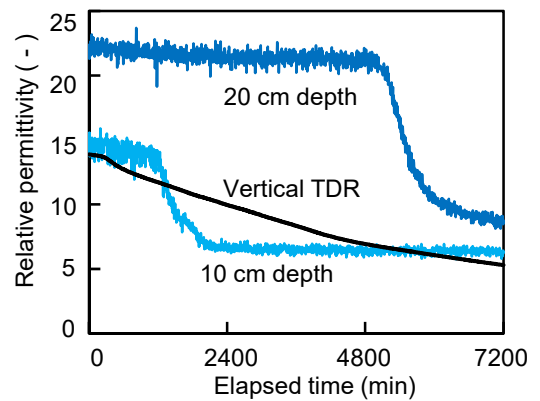
Fig.3 Relative permittivity during freezing.
