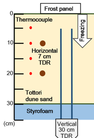
Fig. 1 Schematic of apparatus.
